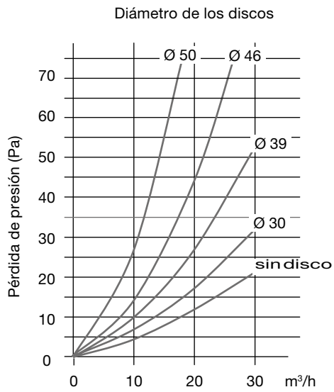
Zehnder ComfoTube 75
