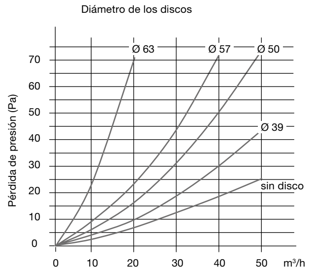
Zehnder ComfoTube 90
